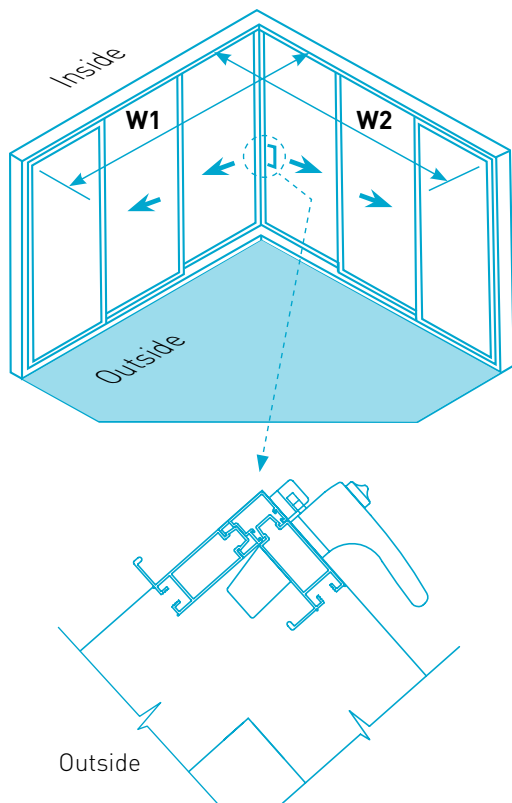
Diagram 1 - Inside Corner
